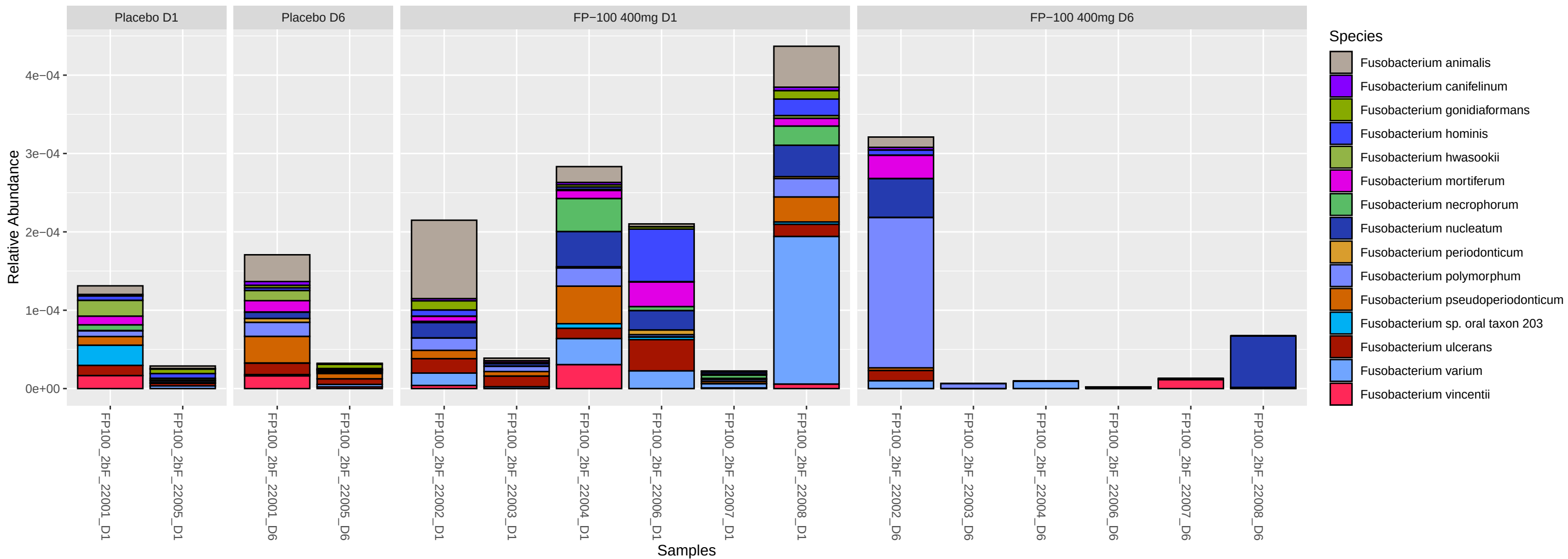
Relative Abundance: Fusobacterium Species
