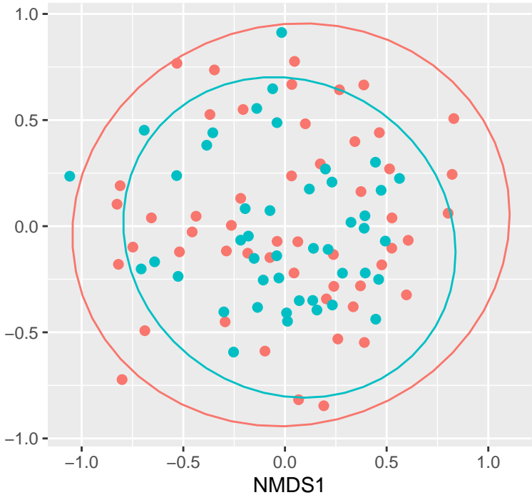
NMDS Plot with Bray–Curtis Dissimilarity Metric
