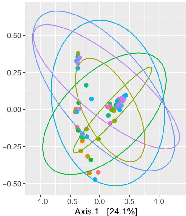
PCoA Plot with Bray–Curtis Dissimilarity Metric
